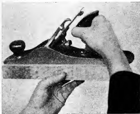
Fig. 30—Using the Sole of the Plane as a Straight-edge
